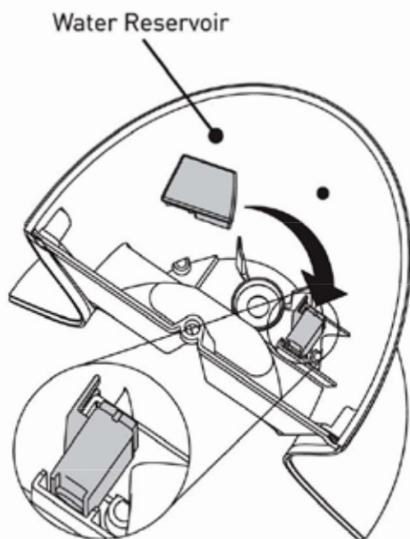
Float Stopper 74-23-2217
